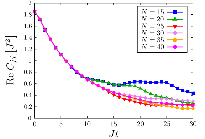
FIG. 3. Real part of real-time current-current correlation function for different number N of sites for G/J = 0.141 , \omega_0/J = 1 , and T/J = 2.5 .
