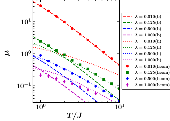
FIG. S1: Mobility obtained from formulas for band transport (labeled "b") and hopping transport (labeled "h") compared with numerically exact HEOM data. Numerical data are presented as points. Results are shown for \omega_0 = J/3 .
