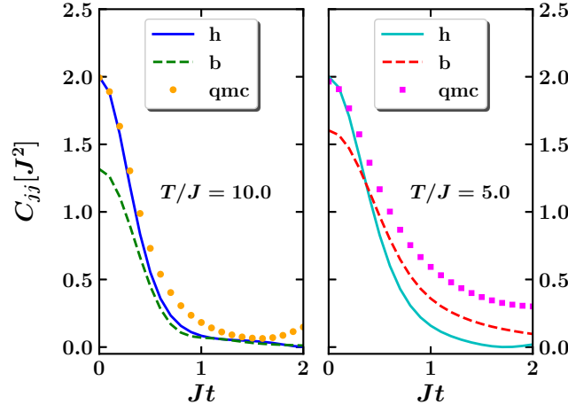
Figure E.7: Real-time current-current correlation functions for \omega_0 = 3J , \lambda = 0.125 , and the temperatures T/J = 5.000 and T/J = 10.000 . Lines labeled with "h" correspond to functions obtained for hopping transport, lines labeled "b" correspond to functions obtained with expression for band transport and QMC results are represented with points.
