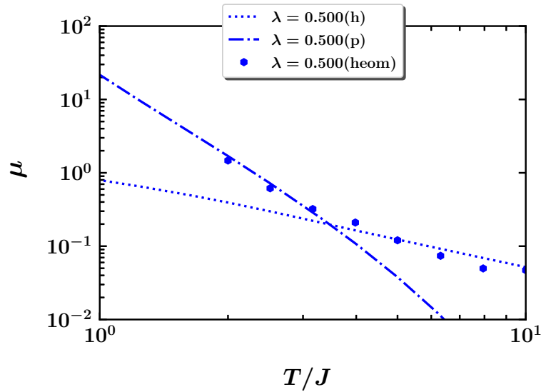
Figure 4.8: Temperature dependence of the mobility for hopping and polaron band transport at \omega_0 = 3J and \lambda = 0.5 . Hopping (“h”) and polaron band transport (“p”) results are compared with numerically exact HEOM data (symbols).
