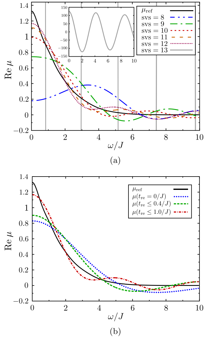
FIG. 1. Examples of the application of the analytic continuation procedure: (a) The reference result (labeled \mu_{\text{ref}} ) and the results obtained using different number of singular values (svs). The inset shows the result obtained using svs = 13 with a full range on the y axis; (b) The reference result ( \mu_{\text{ref}} ) and the results obtained using imaginary-time data only [labeled \mu(t_{\text{re}} = 0) ], using imaginary-time data and real-time data for real times up to 0.4/J [labeled \mu(t_{\text{re}} \leq 0.4/J) ] and using imaginary-time data and real-time data for real times up to 1/J [labeled \mu(t_{\text{re}} \leq 1.0/J) ]. The results are presented for model parameters \omega_0/J = 1 , G/J = 1 and T/J = 1 . The results are shown for \omega \geq 0 because the equality \text{Re}\mu(\omega) = \text{Re}\mu(-\omega) holds.
