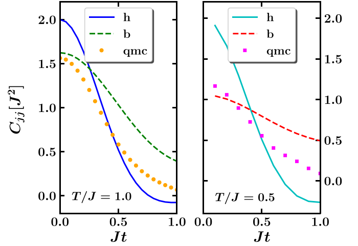
FIG. 11. Real-time current-current correlation functions for \omega_0 = J , \lambda = 0.500 , and the temperatures T/J = 1.000 and T/J = 0.500 . Lines labeled with “h” correspond to functions obtained for hopping transport, lines labeled “b” correspond to functions obtained with expression for band transport, and QMC results are represented with points.
