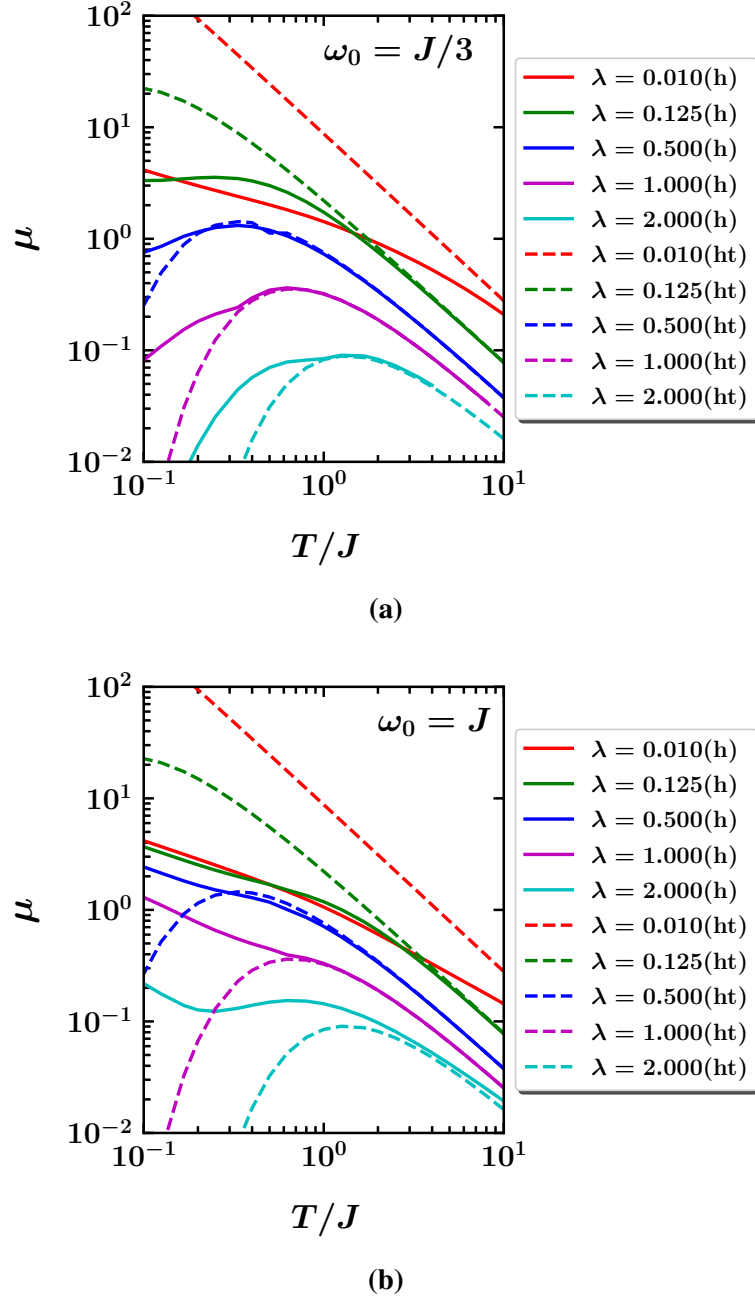
Figure 4.1: Temperature dependence of the hopping mobility for different interaction strengths \lambda . Results obtained from Eq. (4.10) are shown with solid lines (label “h”), while the high-temperature approximation given by Eq. (4.4) is shown with dashed lines (label “ht”). Panel (a) corresponds to \omega_0 = J/3 and panel (b) to \omega_0 = J .
